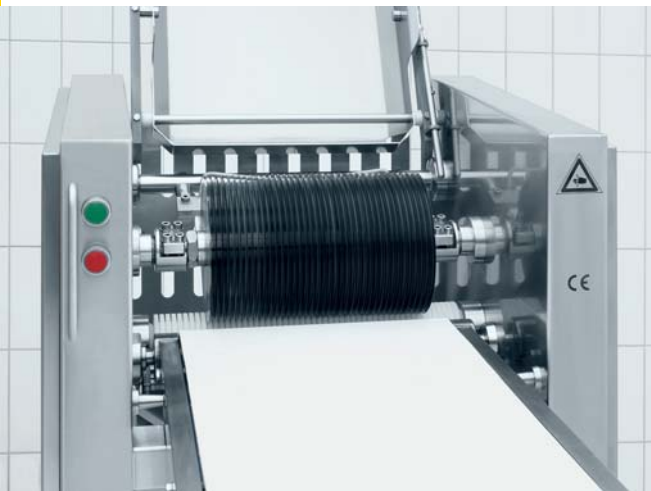
Safety cover opened, transport roller made of synthetic material with stainless steel core (optional)
